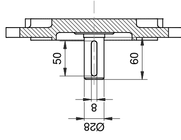
Shaft detail
