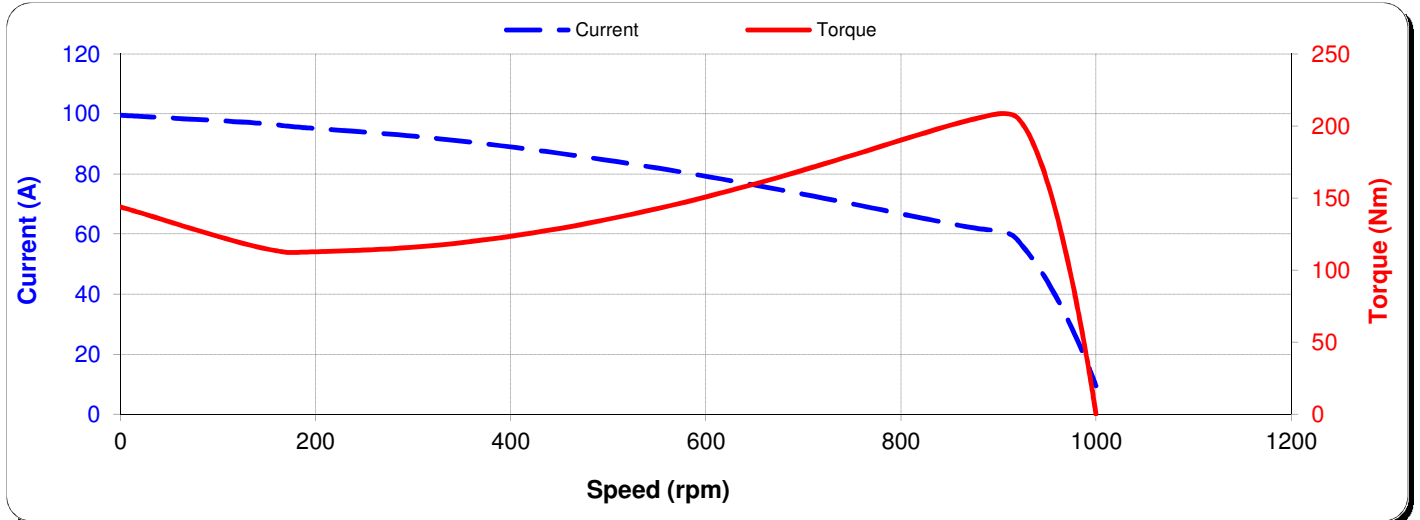
Current and torque versus speed
