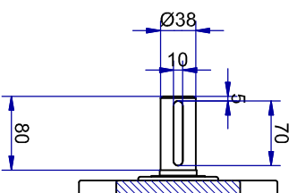
Shaft detail
