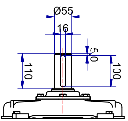
Shaft detail
